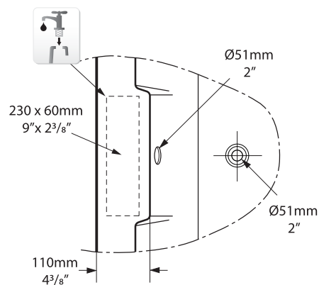
Rim Detail
